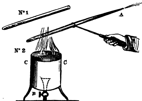
Fig. 157. No. 1. Tube closed at one end, containing tartrate of lead. No. 2. Ditto, closed and drawn out to a capillary tube at A, and held over the mixed gas and air flame obtained by allowing coal gas to escape gently from the cock B into the iron cylinder C C, open at the bottom, and covered with wire gauze at the top, where the mixture of gas and air burns.
